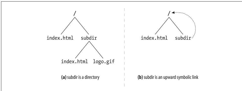
Figure 9-3. Symbolic link cycles
