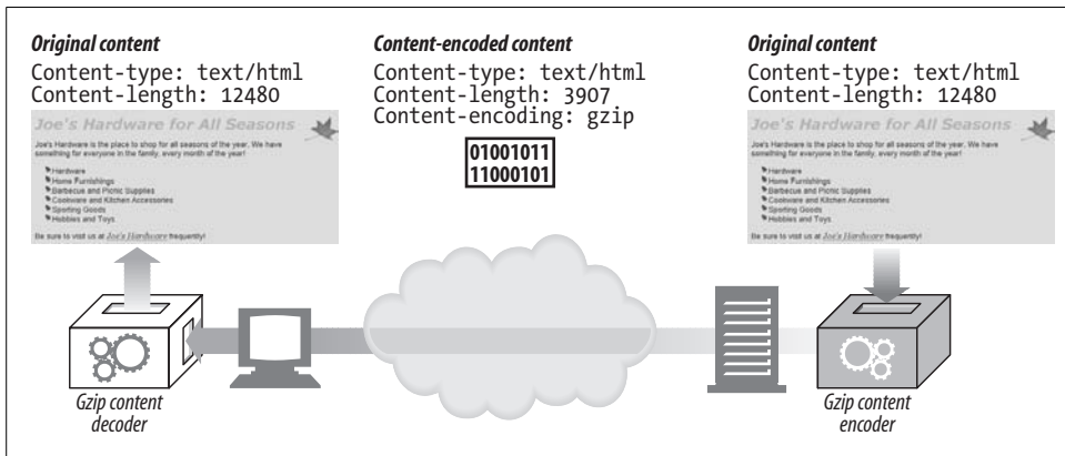
Figure 15-3. Content-encoding example
